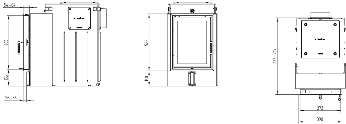
Front panel 37/50G - 830 x 480 mm
