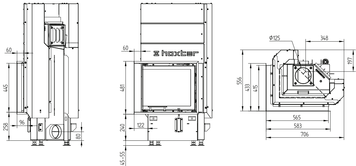
Cover frame 50/35/45Lh left liftdoor 4sides 60 mm 1 x 90°
