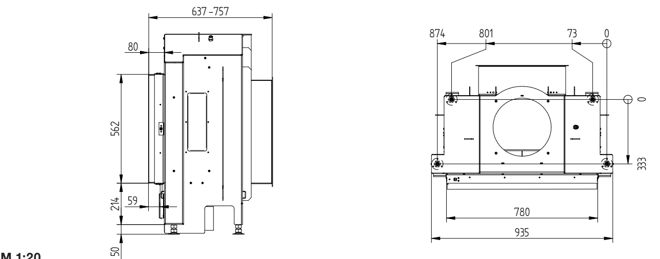
Build-on frame 78/57 side opening 4sides 80 mm / feet
