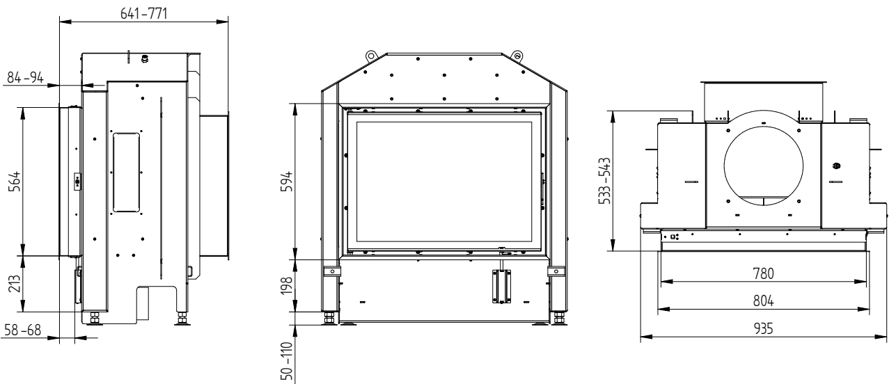
Build-on frame 78/57 side opening 4sides 80 mm / feet
