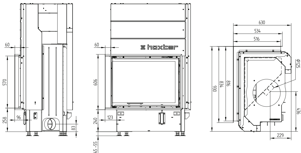
Cover frame 76/45/57Lh left liftdoor 4sides 1 x 90° 60 mm
