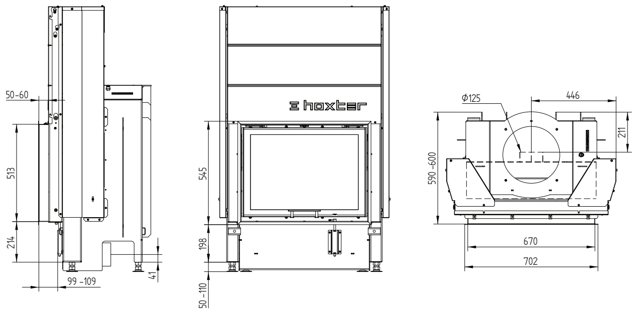
Cover frame 67/51h liftdoor 4sides 80 mm 1 x 90°
