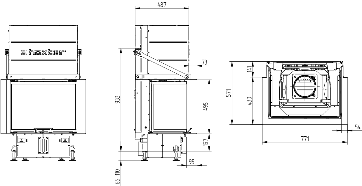
UKA 35/60/35/50Sh supporting construction incl. build-on frame 3sides 70 mm
