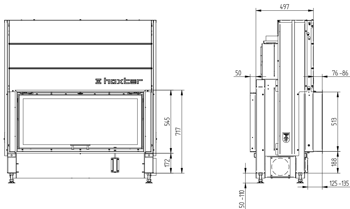
Cover frame 110/51 4sides 1 x 90°, 80 mm
